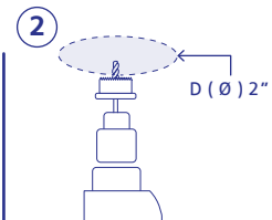
Drill in the selected location for embedding
